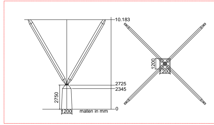
detail kolom Hall 7
